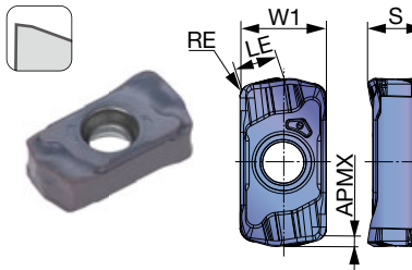
LNMU03UER-ML (for low cutting force, low approach angle)
